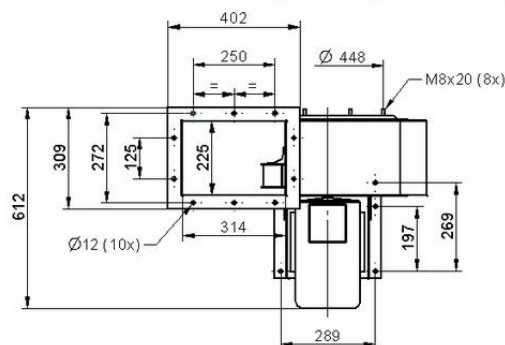
NCF 30/25 Duct inlet diameter 315 mm Duct outlet diameter 400 mm
