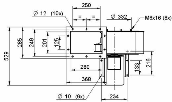
NCF 30/15 Duct inlet diameter 250 mm Duct outlet diameter 315 mm
